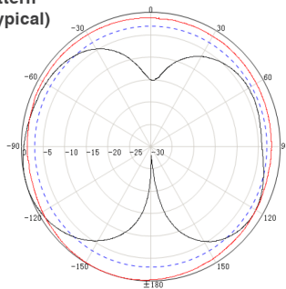
Radiation Pattern High Band (Typical)
